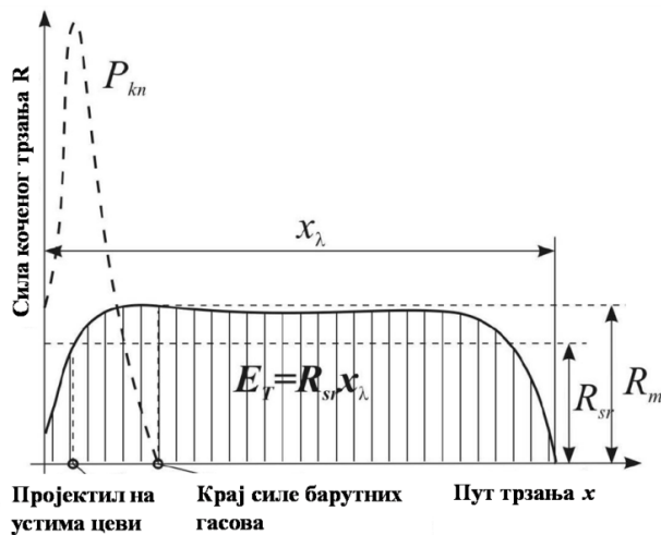
Figure 2. Diagram of recoil braking force [ ]
