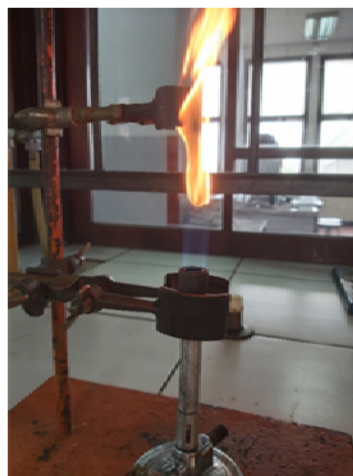
Figure 7. Standard and laboratory setup of apparatus (right) for vertical testing of thermal stability of samples [10]
