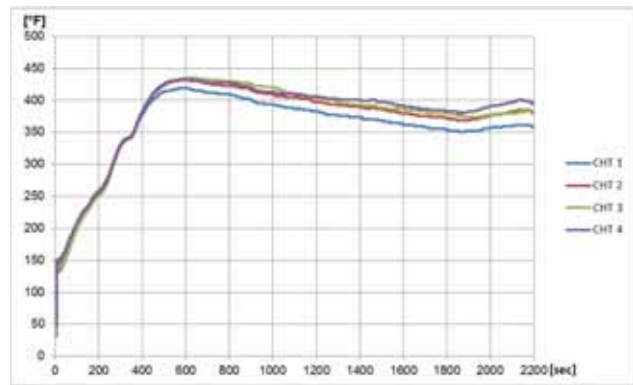
Figure 6. CHT at 65 [kts]
