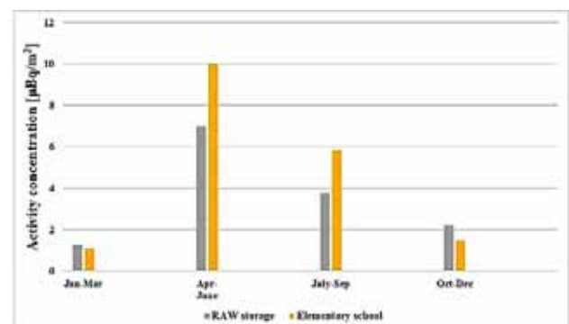
Figure 3. Activity concentration of ^{90}\text{Sr} in air in \mu\text{Bq/m}^3 for different locations during the four quartals of 2021
