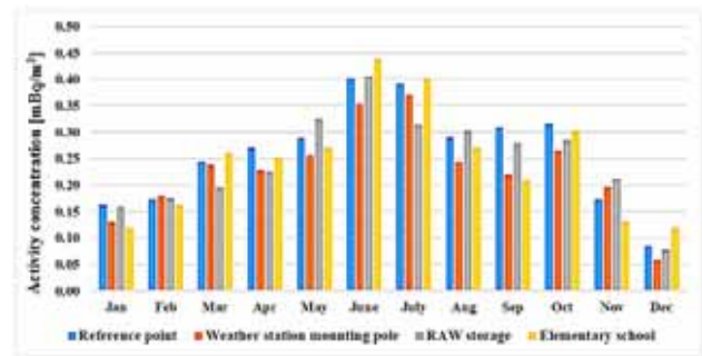
Figure 1. Activity concentration of ^7\text{Be} in air in \text{mBq/m}^3 for different locations during the year of 2021
