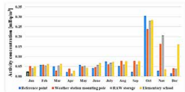
Figure 2. Activity concentration of ^{210}\text{Pb} in air in \text{mBq/m}^3 for different locations during the year of 2021. The framed bar ( \square ) represents MDA, since the value is below MDA
