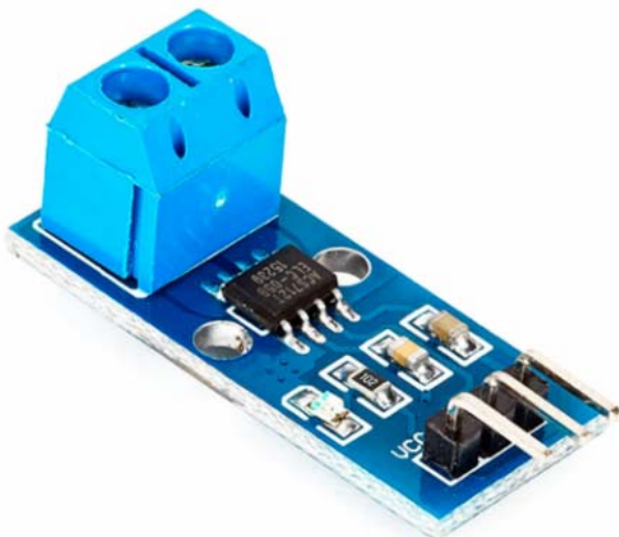
Figure 5. ACS712 current sensor module
