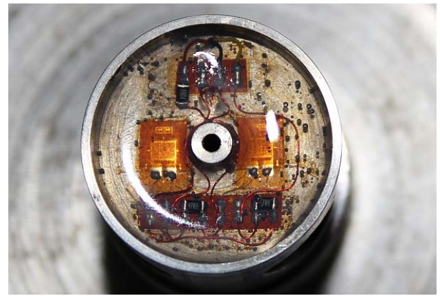
Figure 6. Stagnation temperature strain-gauge transducer
