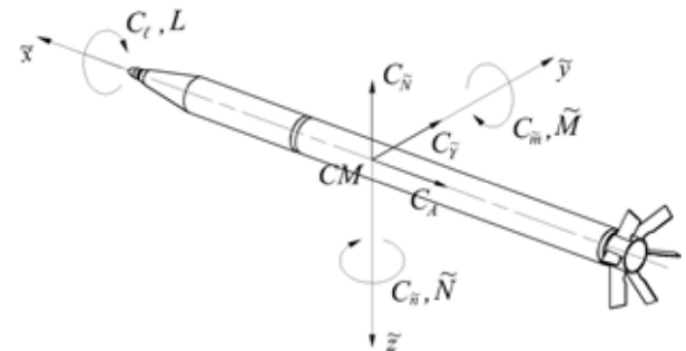
Figure 6. Aerodynamic forces and moments in aeroballistic axis system
